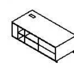
LS-RT1860S W1800×D600×H542 LS-RT1880D W1800×D800×H542
