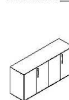
VC-C1675W/G W1600XD450XH750
