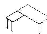
VC-RT1280 W1200XD800XH750
