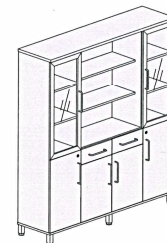
2G4W-5 Cabinet W1600 × D420 × H1800
