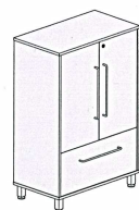
S2F1D-5 Storage W800 × D450 × H1200
