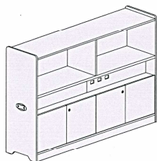
PCA (one side for one person) Partition Combination Cabinet W1800 × D450 × H1200
