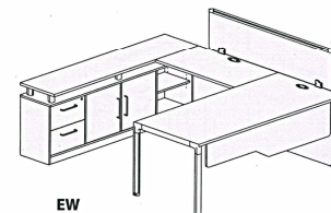
EW Executive Workstation 1600 × 800 (1600 × 2370) 1800 × 900 (1800 × 2470) 2000 × 900 (2000 × 2470)
