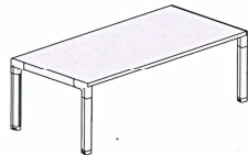
CT2 Coffee Table W1200 × D600 × H450
