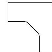
LT-2 L型台面 L shape Table Top W1500/600xD1500/600xT25 W1600/600xD1600/600xT25 W1800/700xD1800/700xT25
