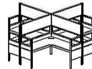
Four Persons Workstation (with glass) M60-4PR-1515 W1500/600"D1500/600"H1650
