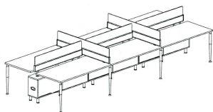
Six Persons Workstation M6B-6P1D-1507 W1500×D700×H750 M6B-6P1D-1608 W1600×D800×H750 M6B-6P1D-1809 W1800×D900×H750
