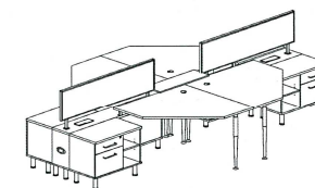
Four Persons Workstation M6B-4P5C-0909 W900×D900×H750 M6B-4P5C-1010 W1000×D1000×H750 M6B-4P5C-1212 W1200×D1200×H750
