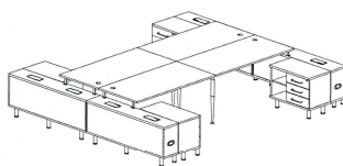
Four Persons Workstation M6B-4P2A-1507 W1500×D700×H750 M6B-4P2A-1608 W1600×D800×H750 M6B-4P2A-1809 W1800×D900×H750
