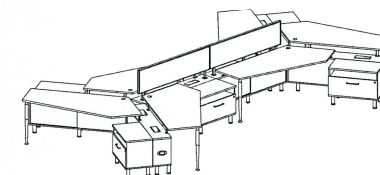
Six Persons Workstation M6B-6P4E-1507 W1500×D700×H750 M6B-6P4E-1608 W1600×D800×H750 M6B-6P4E-1809 W1800×D900×H750
