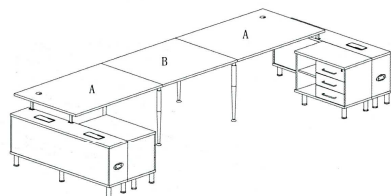
Three Persons Workstation M6B-3P2C-1412 W1400×D1200×H750 M6B-3P2C-1212 W1200×D1200×H750
