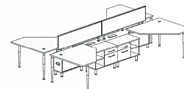
Four Persons Workstation M6B-4P5B-0909 W900×D900×H750 M6B-4P5B-1010 W1000×D1000×H750 M6B-4P5B-1212 W1200×D1200×H750
