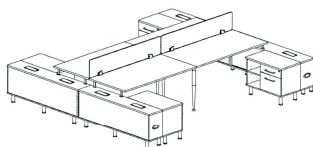
Four Persons Workstation M6B-4P2B-1507 W1500×D700×H750 M6B-4P2B-1608 W1600×D800×H750 M6B-4P2B-1809 W1800×D900×H750
