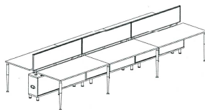
Six Persons Workstation M6B-6P1C-1507 W1500×D700×H750 M6B-6P1C-1608 W1600×D800×H750 M6B-6P1C-1809 W1800×D900×H750
