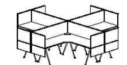
Four Persons Workstation MB-4PB-1515 W1500 x D500 x W1500 x D800 x H750 MB-4PB-1515 W1500 x D500 x W1800 x D800 x H750 MB-4PB-1515 W1800 x D700 x W1800 x D700 x H750
