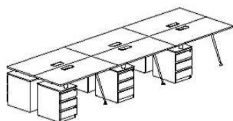
Six Persons Workstation MB-6PB-1507 W1500 x D700 x H750 MB-6PB-1808 W1800 x D800 x H750
