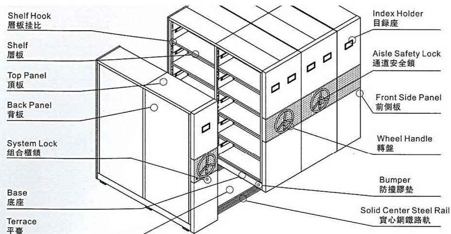
械式活动推柜 DOUBLE COMPACTUS(MECHANICAL TYPE)
